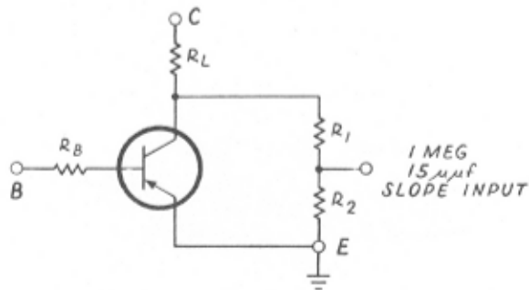
Fig. 2-12. Typical grounded-emitter transistor mounting board circuit.
